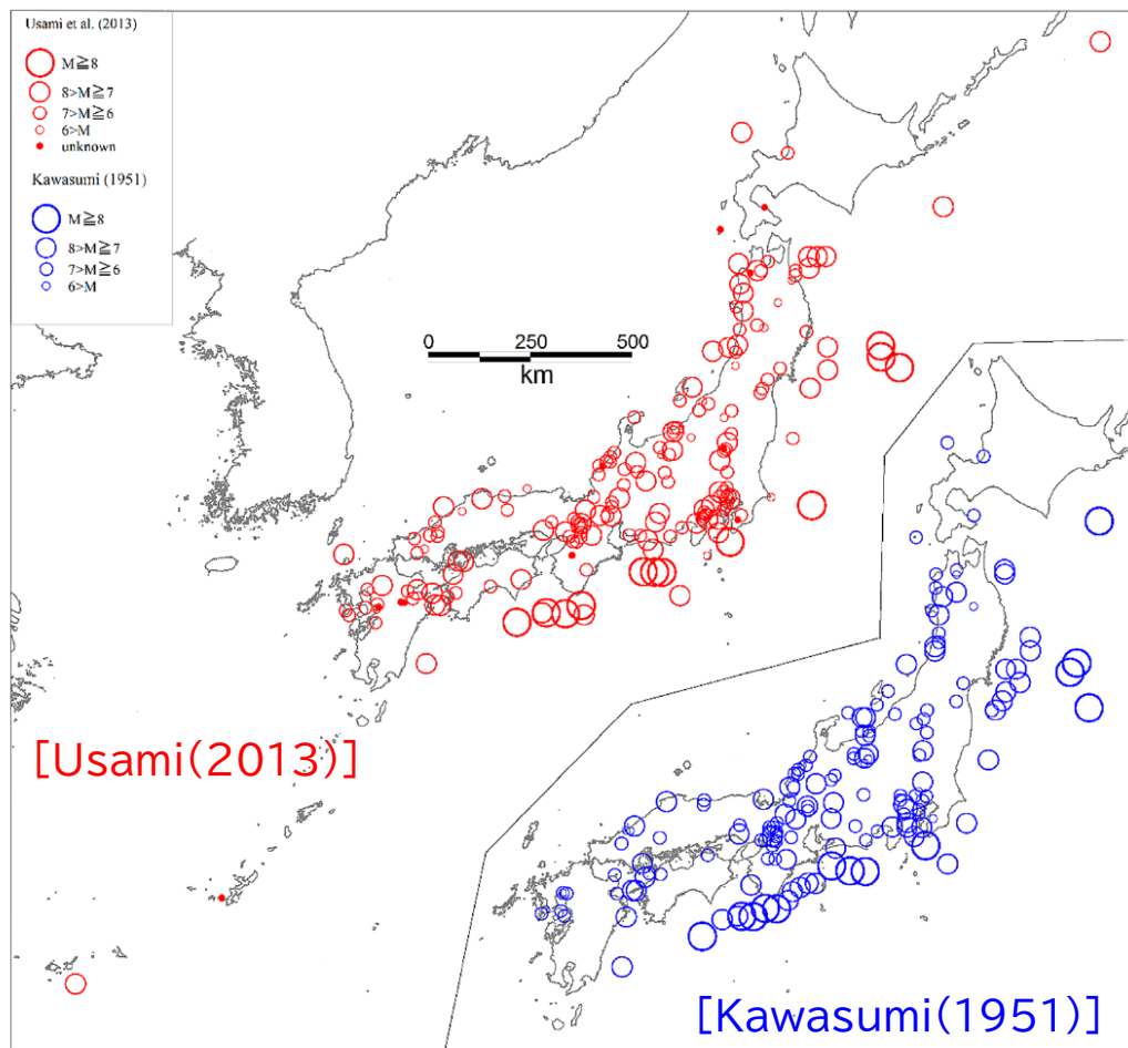
Fig. 3 Epicenter distributions of destructive earthquakes in Japan from 679 AD to 1872 in the latest Usami's list and Kawasumi's list. Red circles are epicenters of 214 events of Usami et al. (2013). Blue circles are epicenters of 167 events in Kawasumi (1951). Mk is transformed to the usual magnitude (M)
